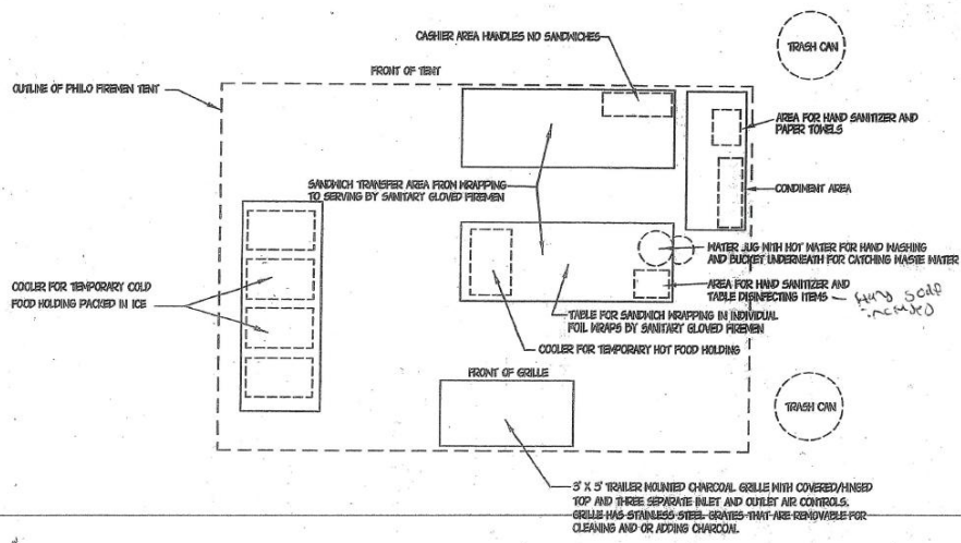
COOKING AND SERVING LAYOUT UNDER TENT SCALE: 1/4"=1'-0"
